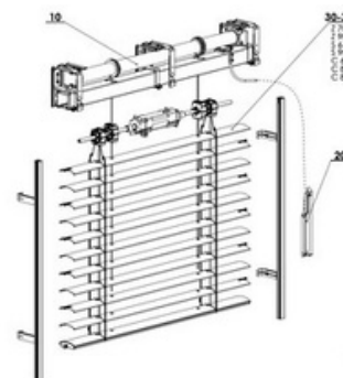
ZETTA 70, ZETTA 90 EXTERIOR BLIND DIAGRAM
