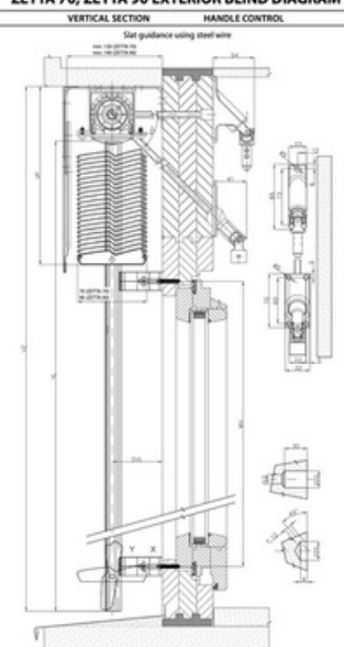
ZETTA 70, ZETTA 90 EXTERIOR BLIND DIAGRAM
